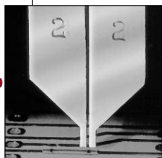
TL-086B Precision Parallel Gap Weld Head
